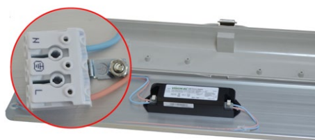
Connection rapide
