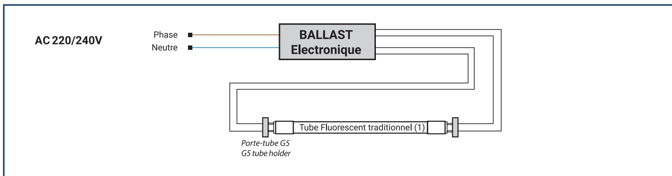
(1) Traditional Fluorescent Tube
